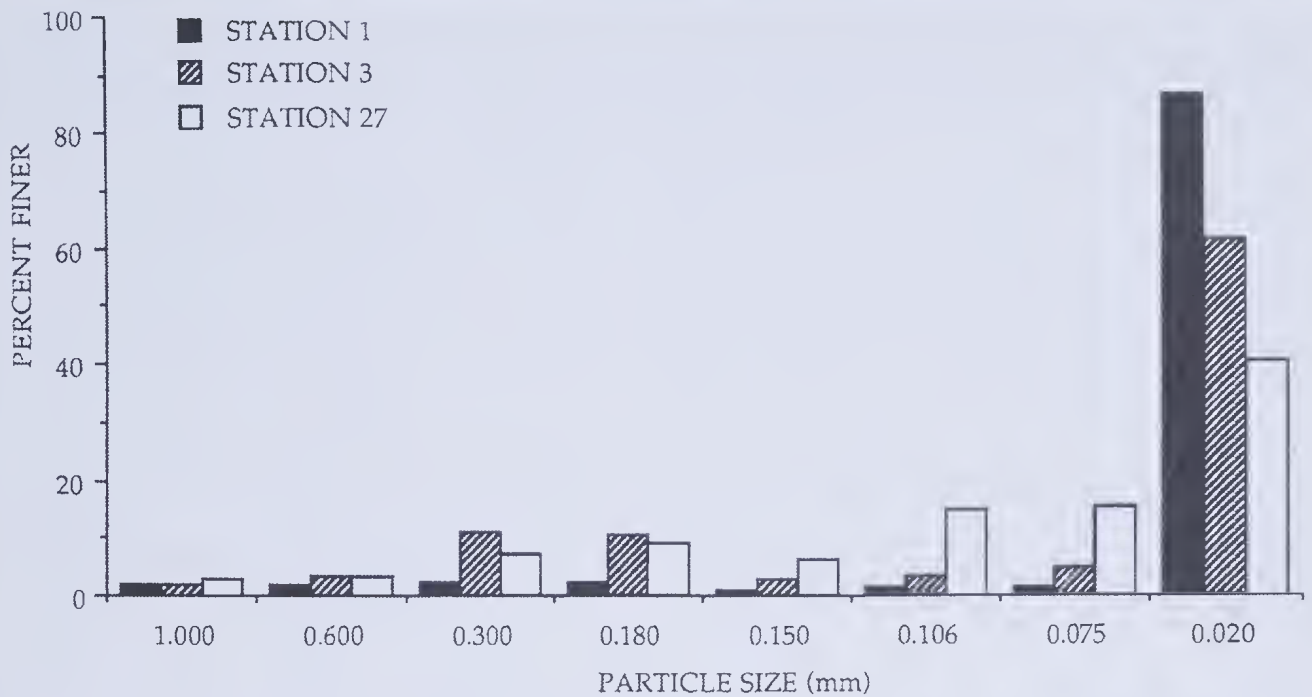
Figure 2. Particle size distribution for sediments from Leschenault Inlet.
